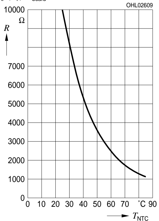
Typische Thermistor Kennlinie 2) 7) Seite 16 Typical Thermistor Graph 2) 7) page 16 I_F = f(V_F); T_{board} = 25\text{ °C}
